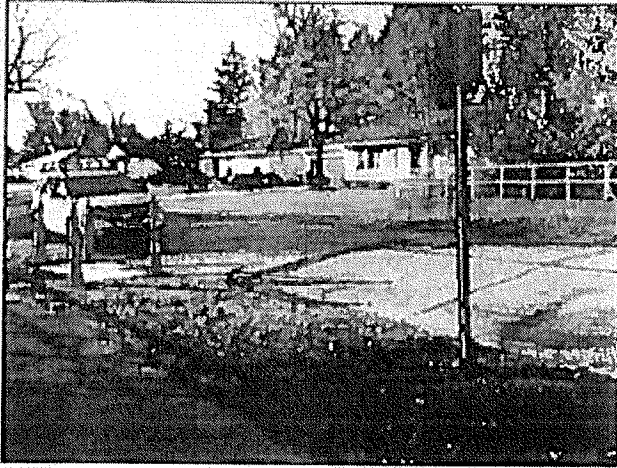
Sinkhole on inlet end is coned off. Cracks around pipe on pavement.
